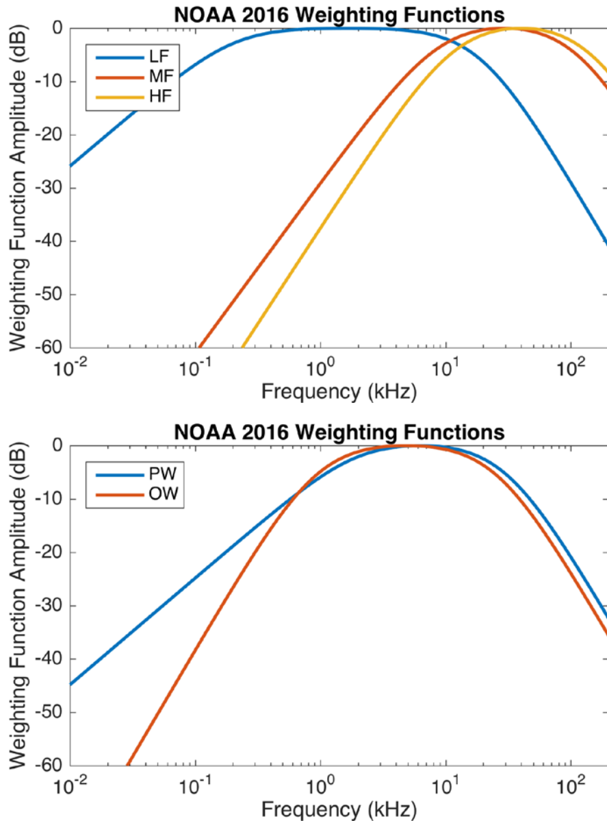
Figure 4-2. Auditory Weighting Functions for Cetaceans (Top Panel: LF, MF, and HF Species) and Pinnipeds (Bottom Panel: PW, OW) (NOAA, 2015, 2016a).
