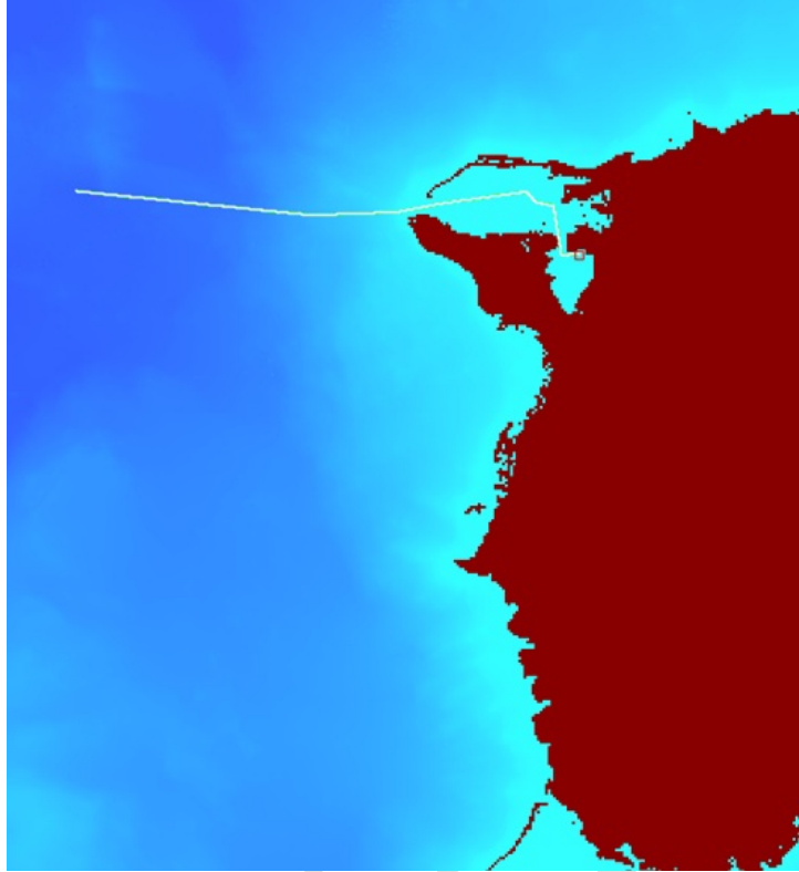
Figure 13. Example Track, Submarine Navigation Waypoints
