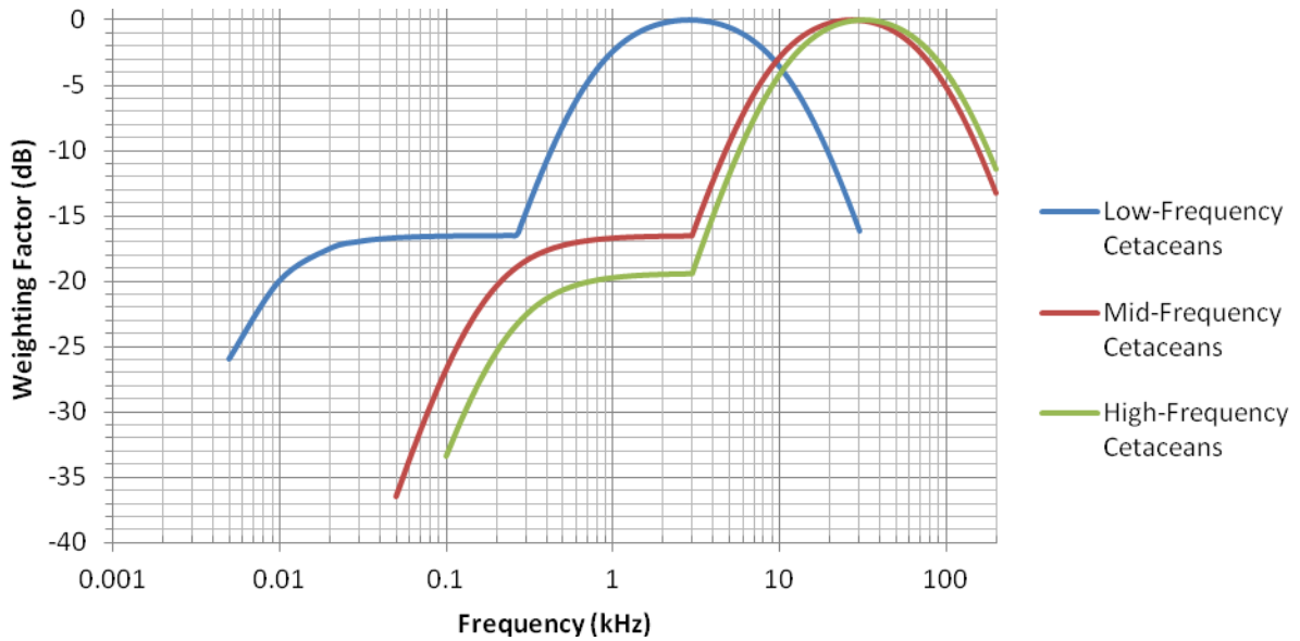
Figure 10. Navy Type II Weighting Functions for Low-, Mid-, and High-Frequency Cetaceans
