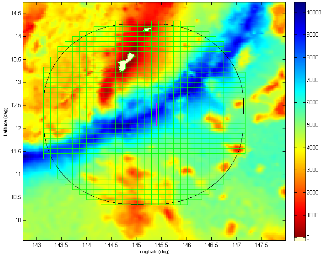
Figure 20. Example Modeling Area
