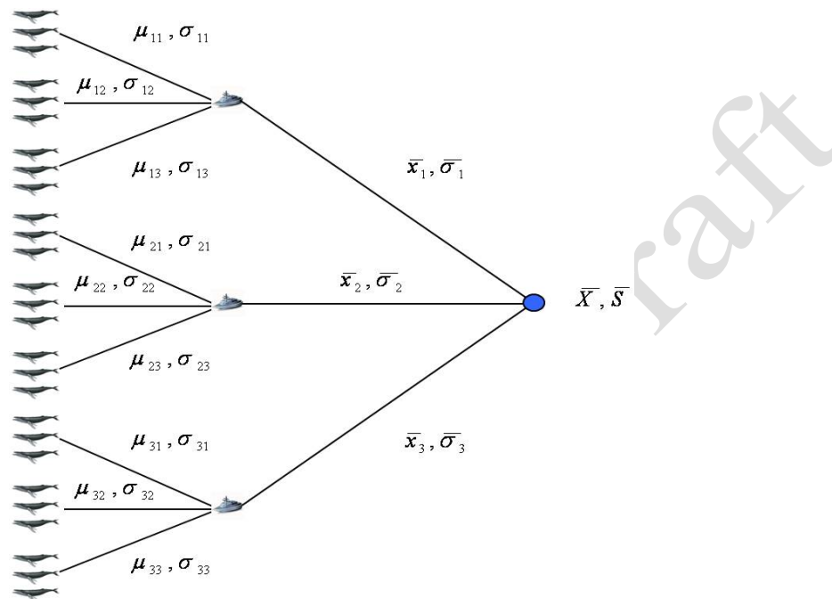
Figure 25. Bootstrapping Approach Used to Calculate Simulation Statistics
