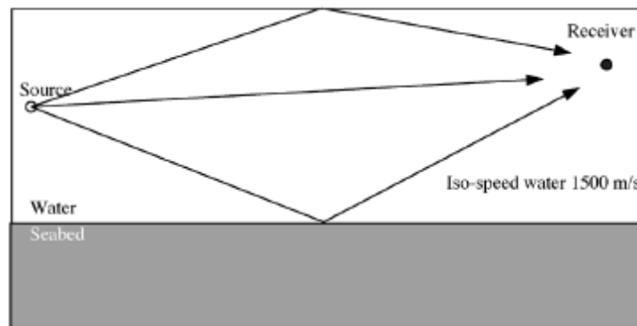
Figure 18. Generalized Pathways of Shock Waves and Sound Energy (adapted from Siderius and Porter, 2006)
