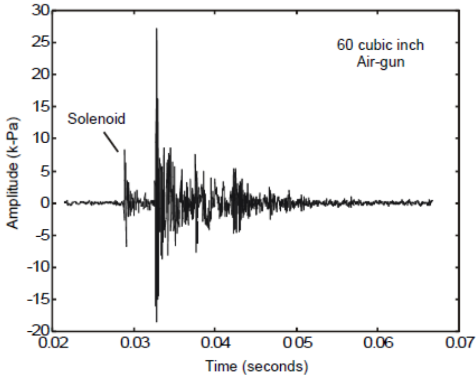
Figure 6. Characteristic Waveform of an Airgun Pulse
