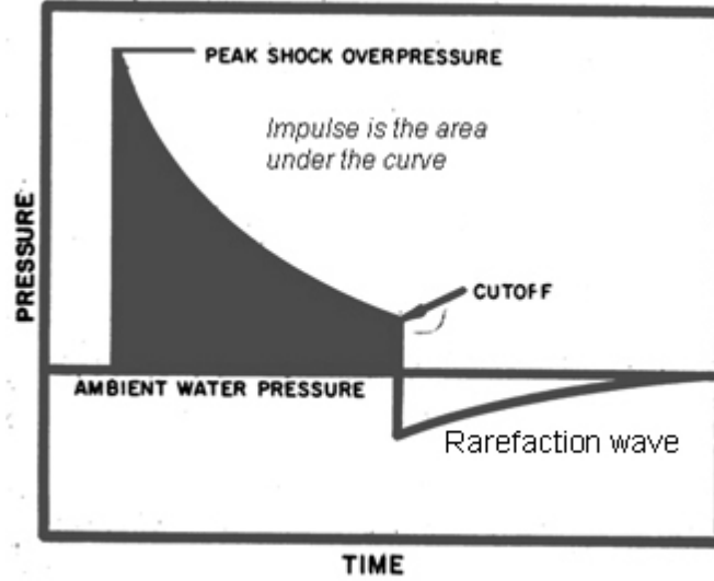
Figure 17. Generalized Shock Wave
