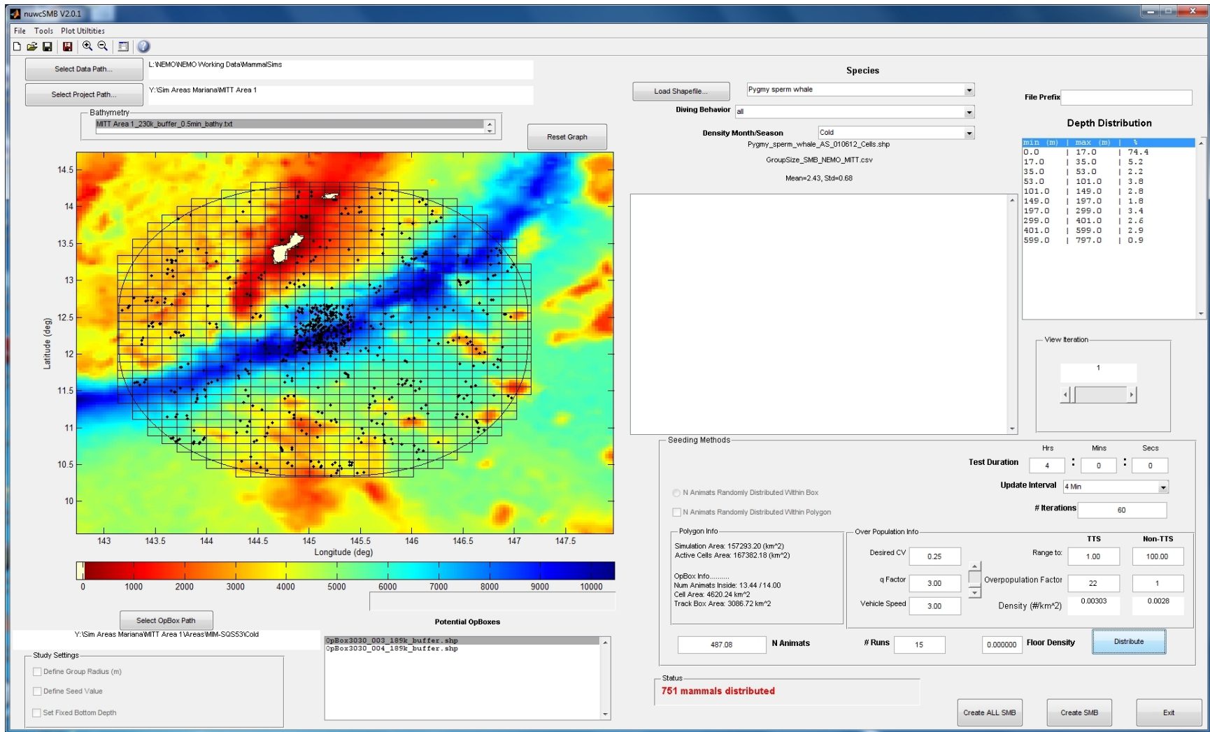
Figure 21. Distribution for Pygmy Sperm Whale in the MITT Area 1 Operating Area During the Cold Season (Black dots represent individual animats)
