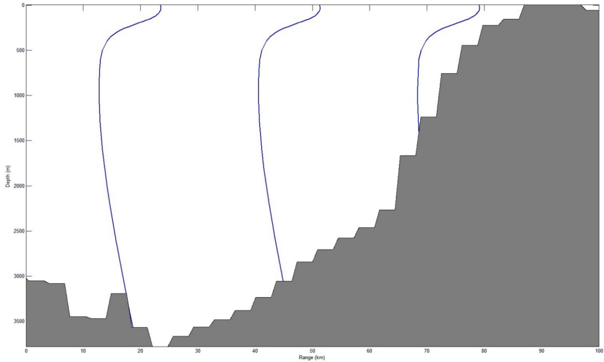
Figure 16. Sample Sound Speed Profiles
