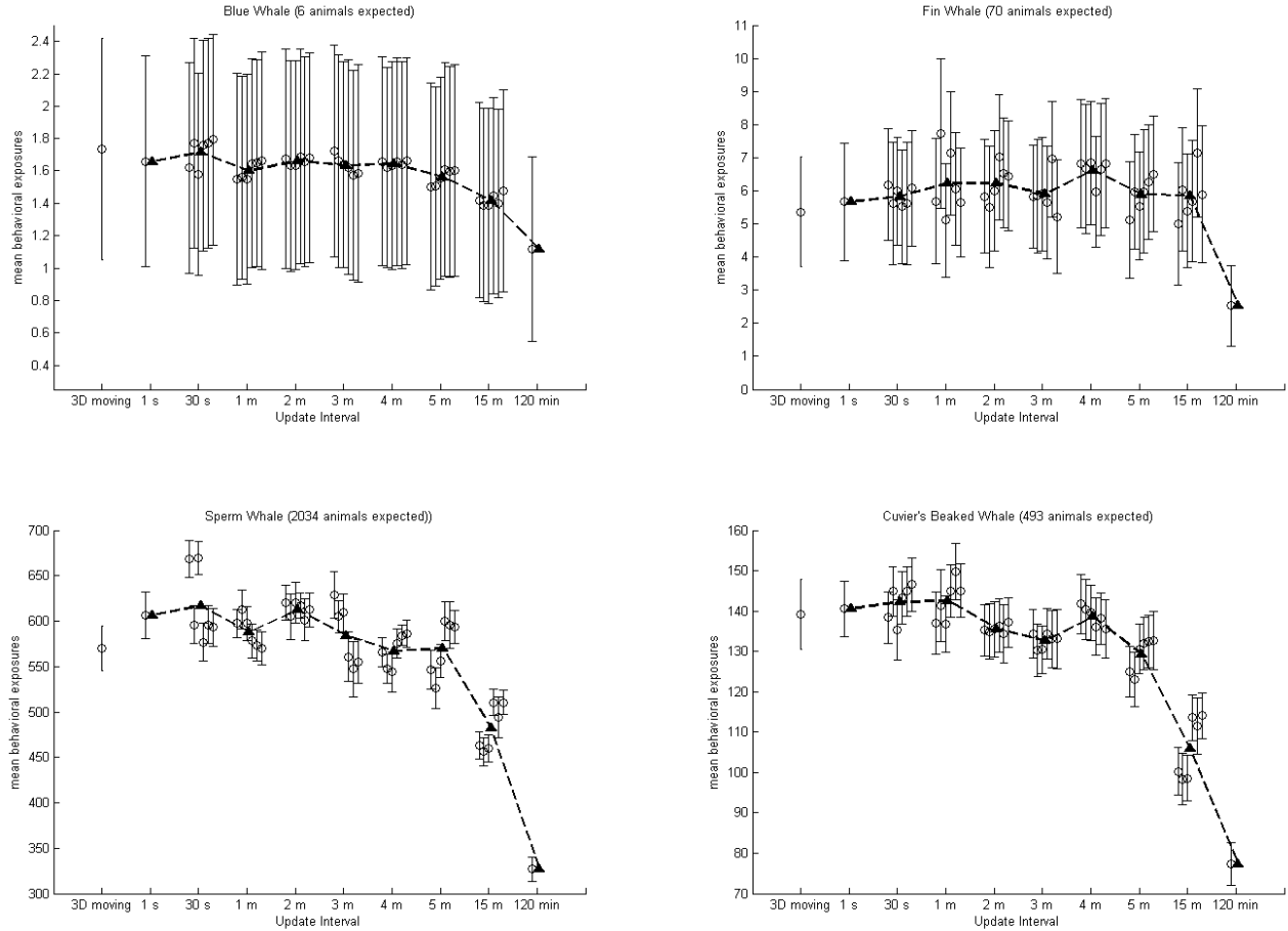
Figure 22. Effect of Update Rate on Estimated Values for Two Shallow-Diving Cetaceans (top row) and Two Deep-Diving Cetaceans (bottom row)
