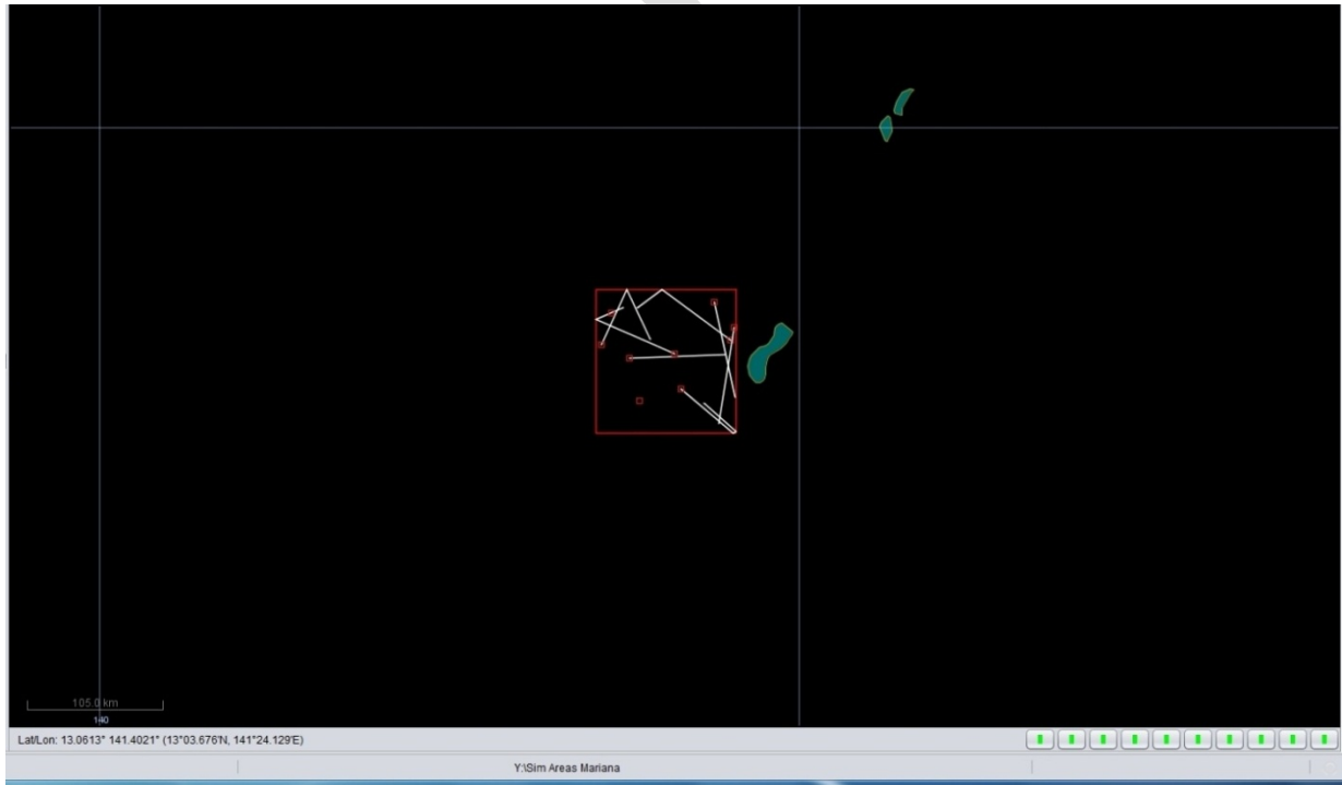
Figure 14. Example Perimeter Bounce
