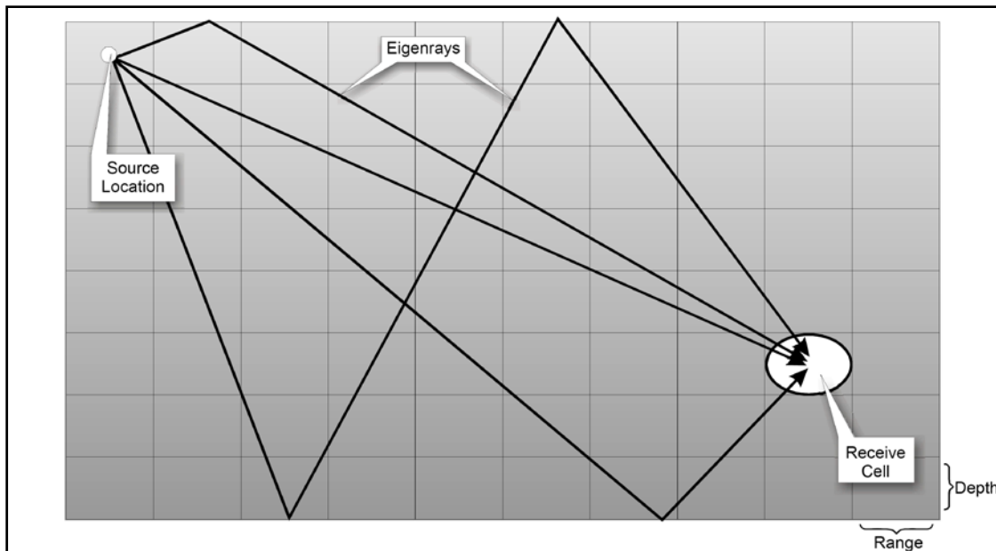
Figure 19. Typical Eigenray Paths for Relatively Short-Range Propagation
