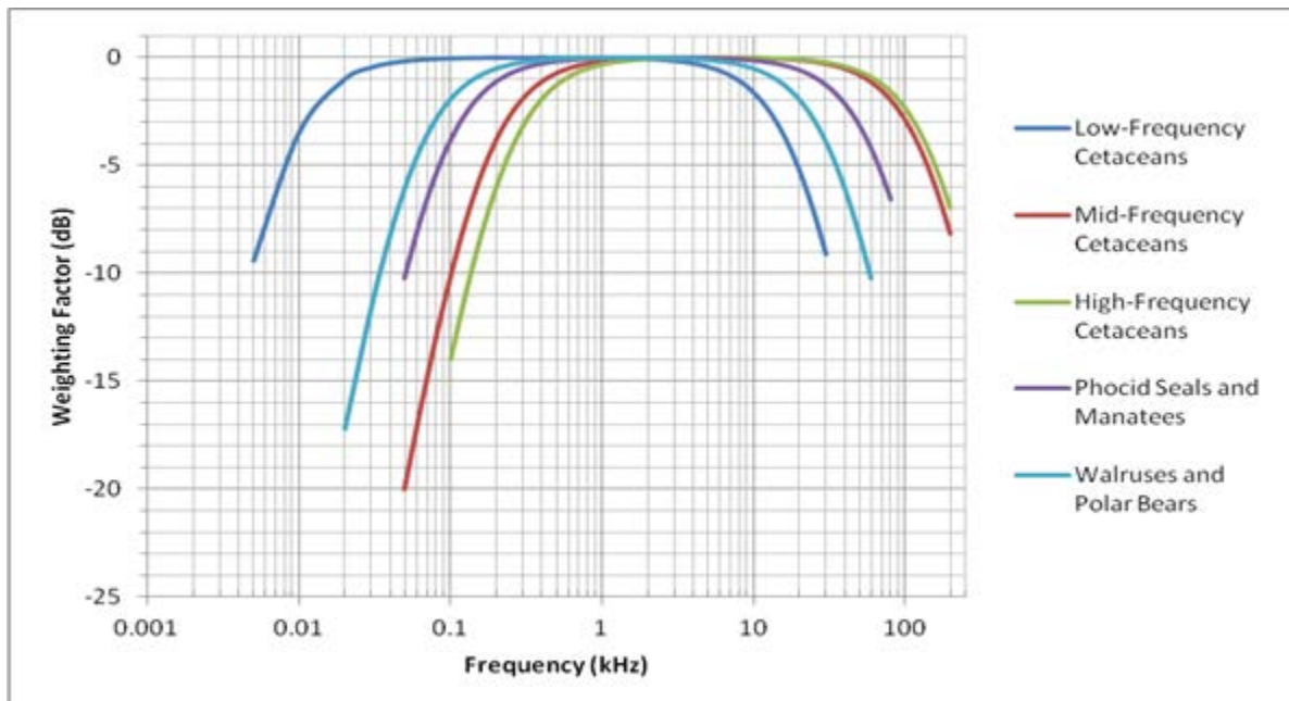
Figure 9. Navy Type I Weighting Functions
