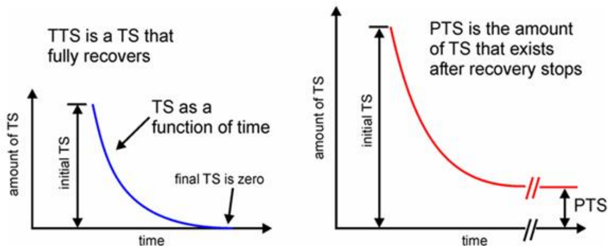
Figure C-2: Two Hypothetical Threshold Shifts
