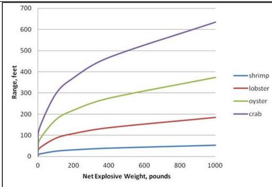
Figure C-3: Prediction of Distance to 90 Percent Survivability of Marine Invertebrates Exposed to an Underwater Explosion
